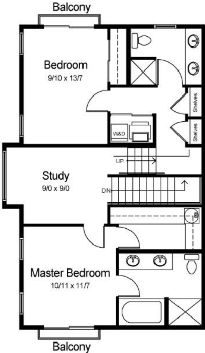
Upper Level 771 Sq. Ft.
