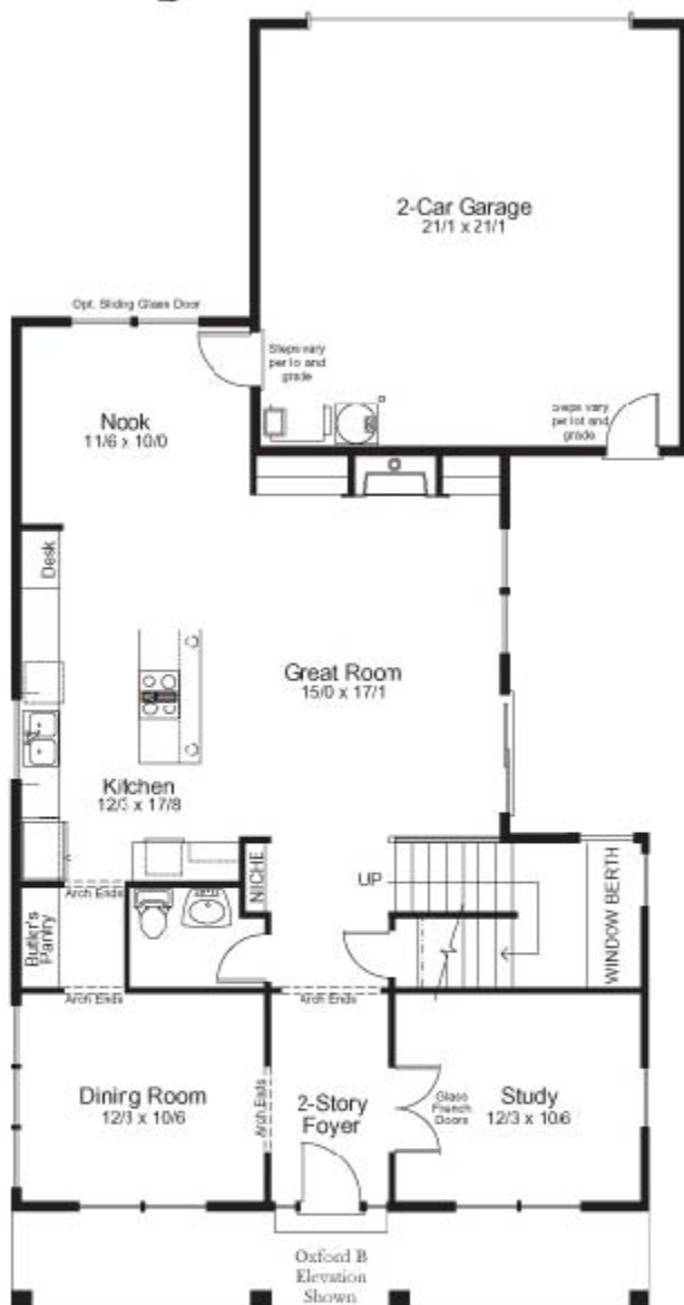
■ MAIN FLOOR PLAN 1176 SQ. FT.
