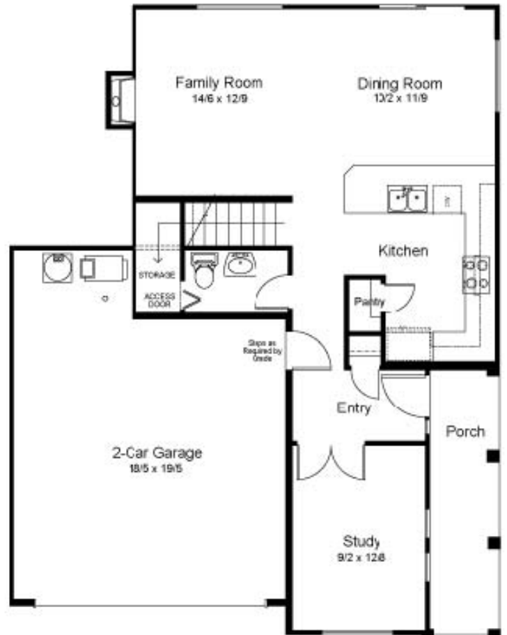
MAIN FLOOR PLAN 798 SQ. FT.
