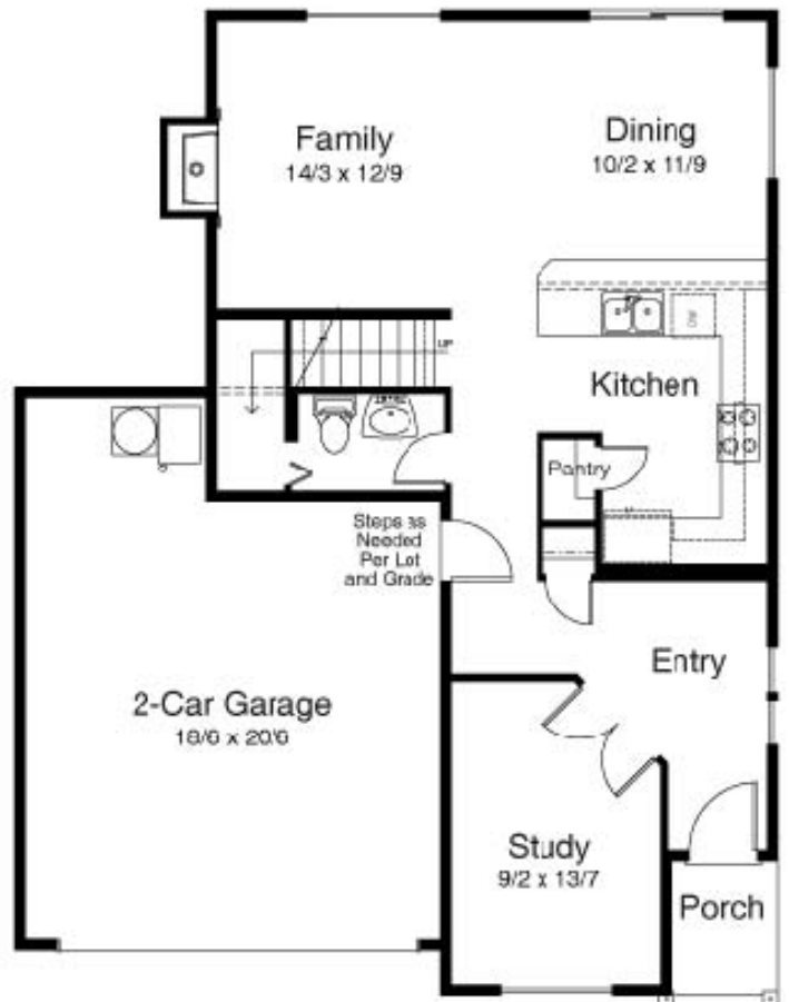
MAIN FLOOR PLAN 858 SQ. FT.
