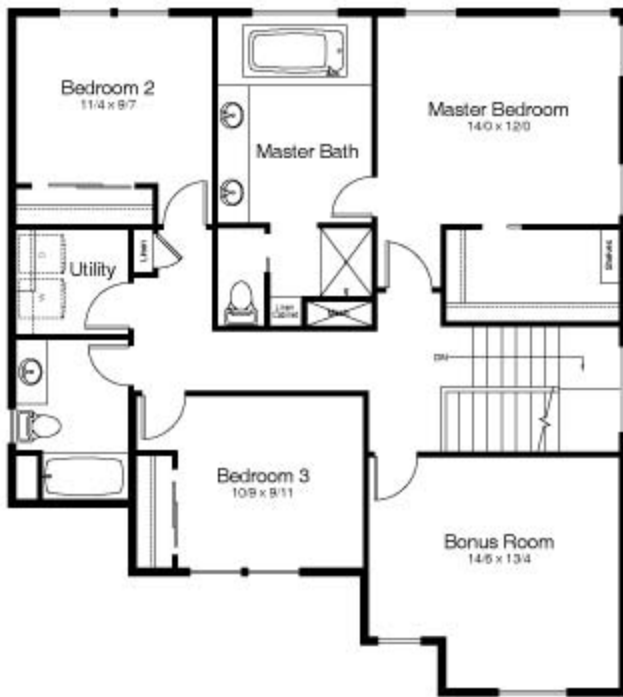
SECOND FLOOR PLAN 1184 SQ. FT.
